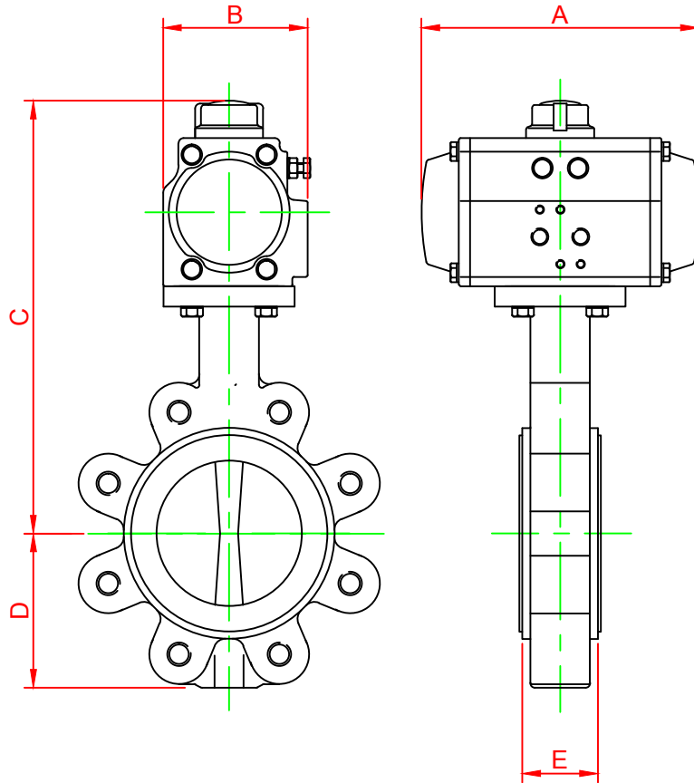
Spring Return - Dimensions
